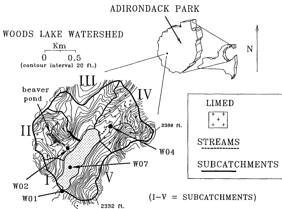
Fig. 2. Map of Woods Lake watershed. Subcatchments II and IV were treated with \text{CaCO}_3 .
